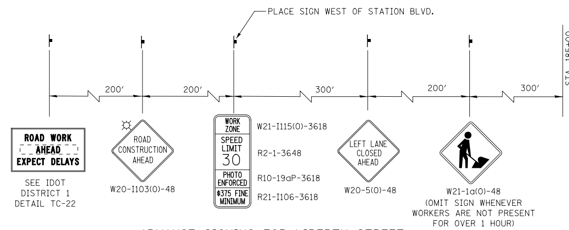
ADVANCE SIGNING FOR LIBERTY STREET (SPACING MAY VARY DUE TO FIELD CONDITIONS)
