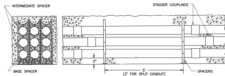
ELEVATION OF MONOLITHIC METHOD
