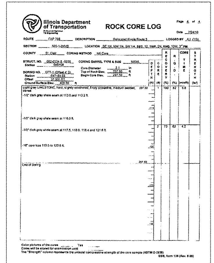
BORING SPT-1 (4 of 4)
