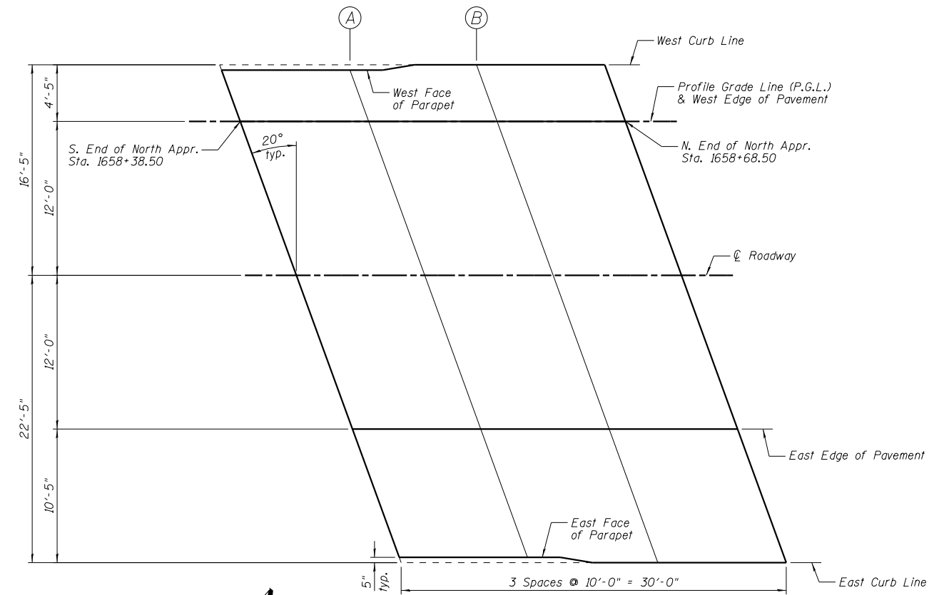
NORTH APPROACH SLAB PLAN
