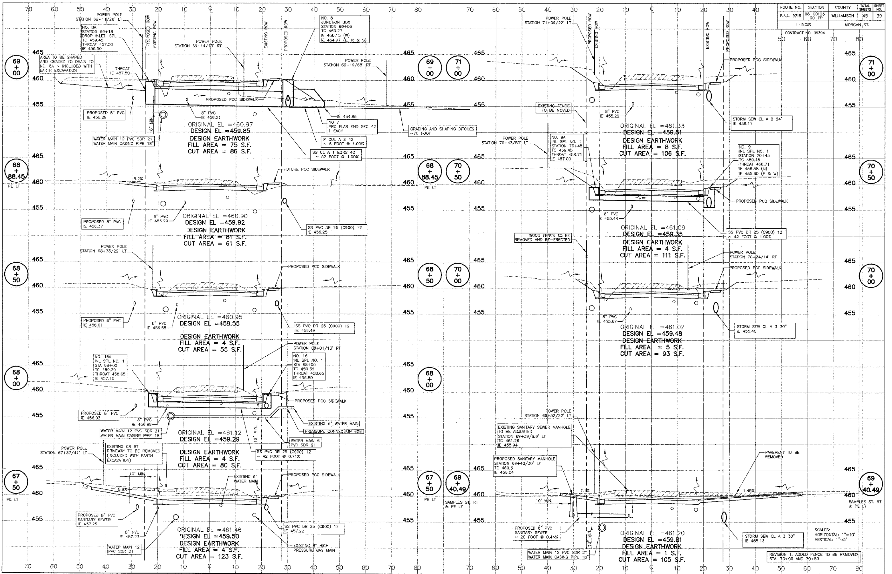
MORGAN AVE. IMPROVEMENTS - CROSS SECTIONS STATION 67+50 TO 71+00
