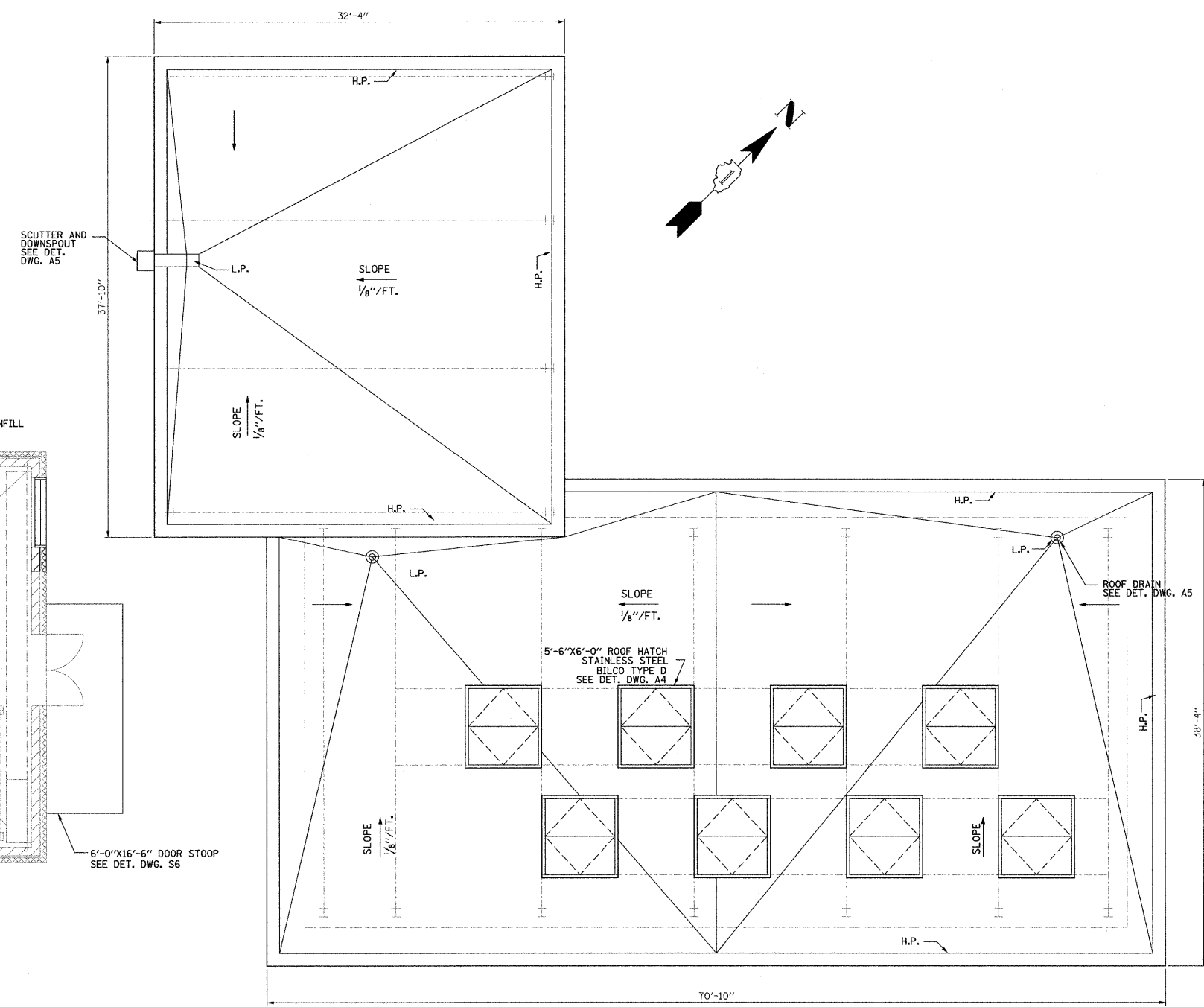
ROOF PLAN
