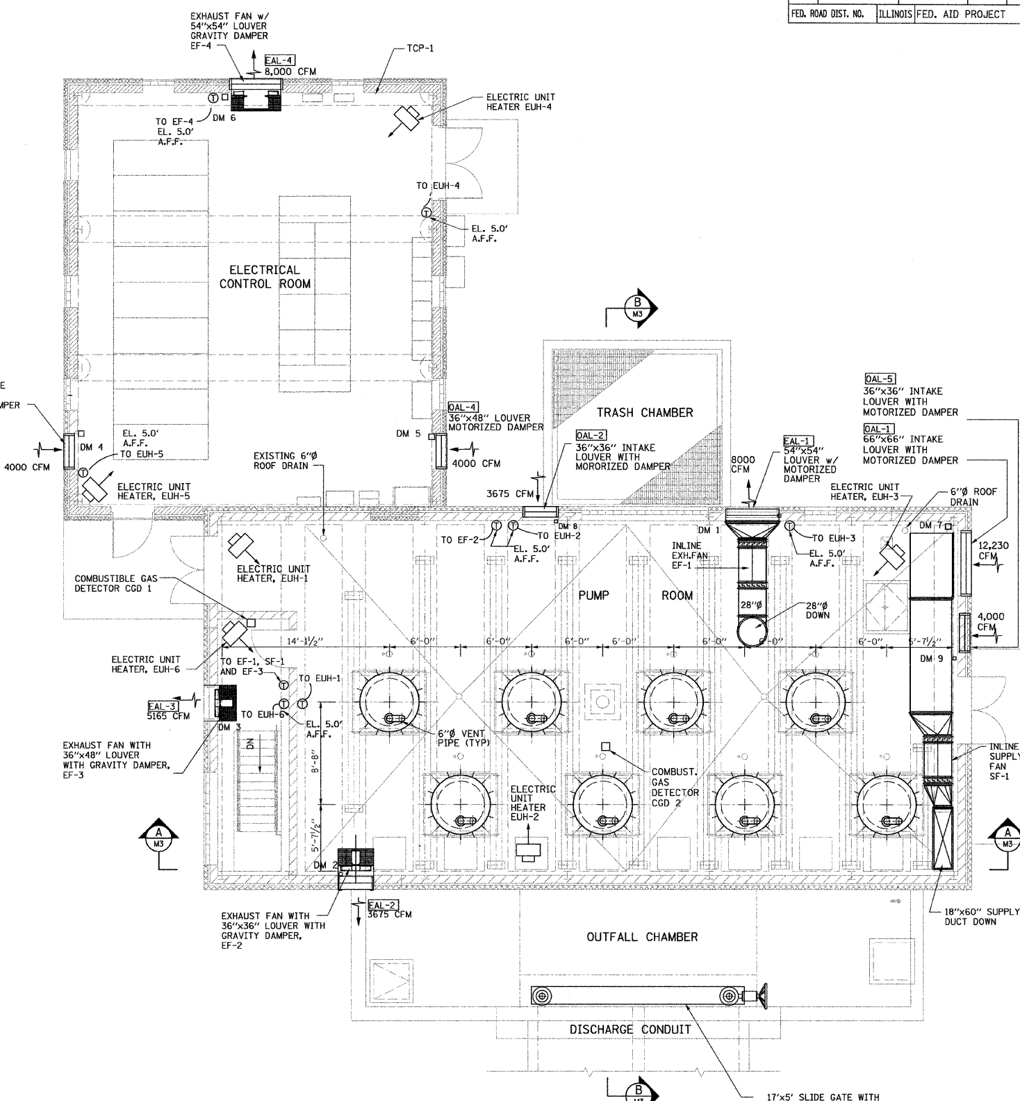
FLOOR PLAN ABOVE EL. +9.5'
