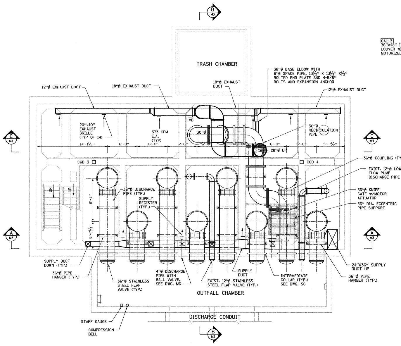
PLAN ABOVE EL. -8.5'
