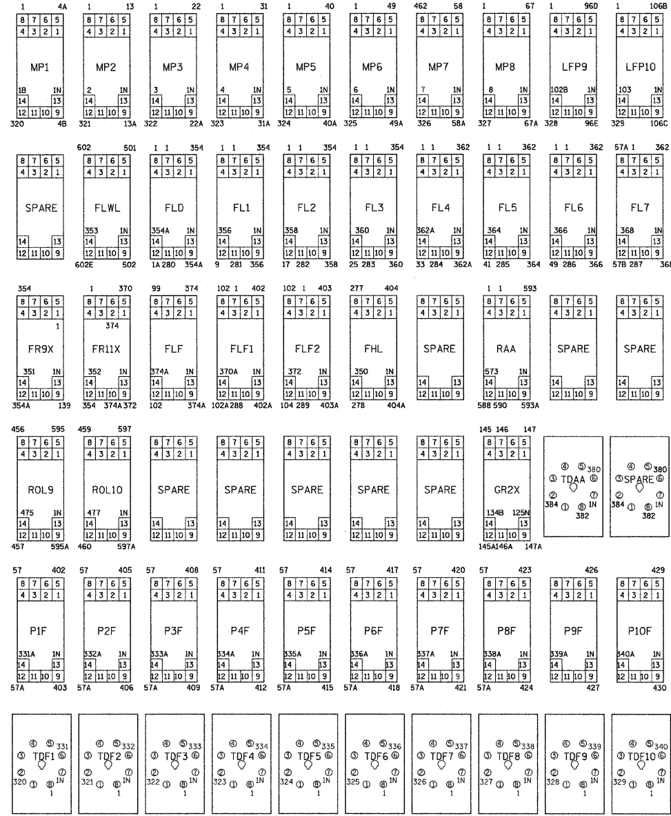
DETAIL A CONTROL RELAYS DWG. E23 EACH RELAY SHALL HAVE AN ENGRAVED NAMEPLATE
