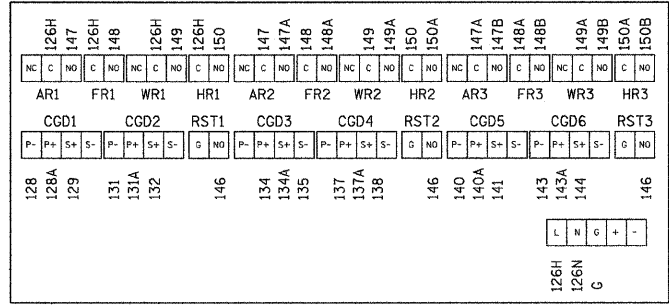
DETAIL D COMBUSTIBLE GAS MONITOR DWG. E23
