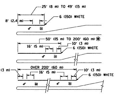
TYPICAL TURN LANE MARKING
