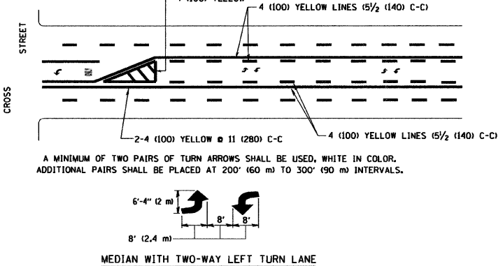
TYPICAL PAINTED MEDIAN MARKING
