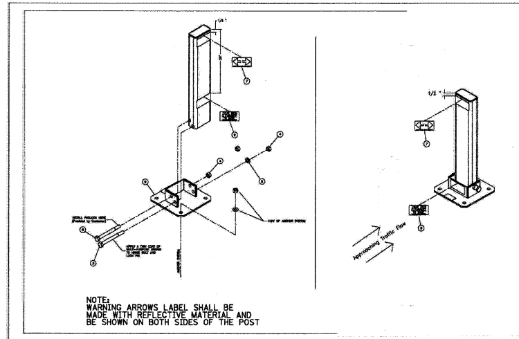
LOCKABLE REMOVABLE POST DETAIL
