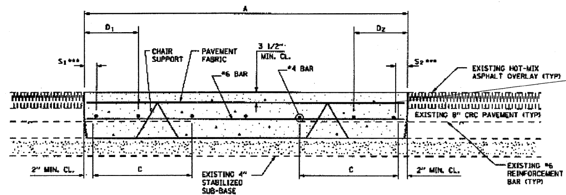
PROPOSED CLASS A PATCHING DETAIL
