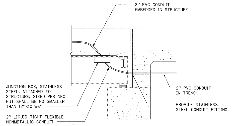
SECTION VIEW AT ABUTMENT
