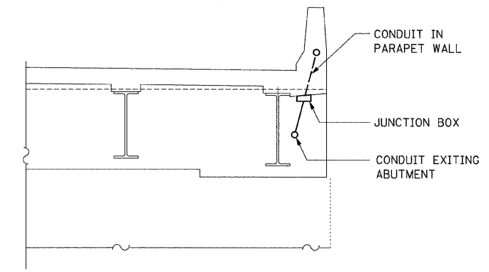
ELEVATION VIEW AT ABUTMENT
