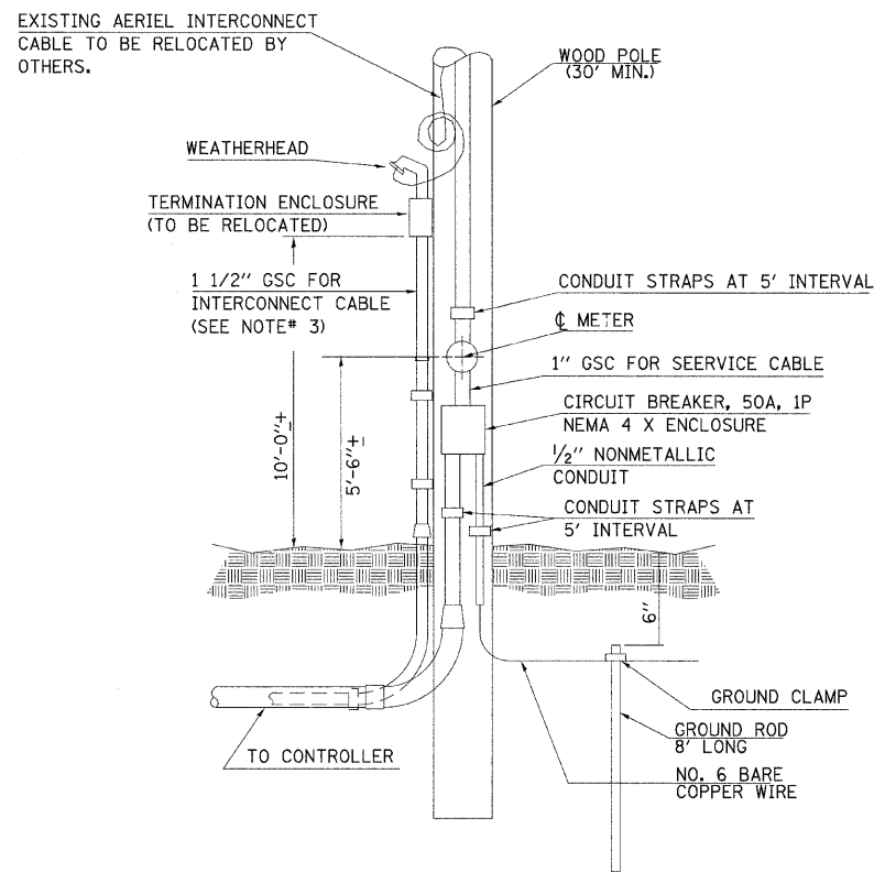
SERVICE INSTALLATION TYPE A
