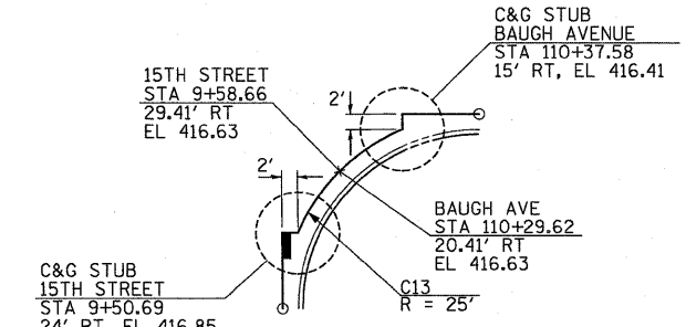
DETAIL "Q"
