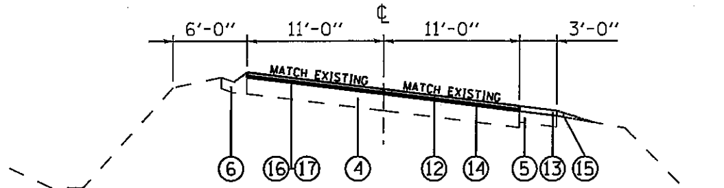
TYPICAL SECTION STA. 70+08.12 TO STA. 80+64.12
