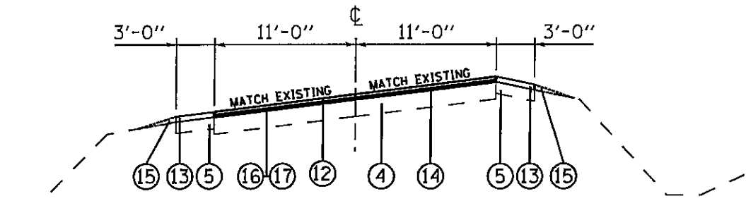
TYPICAL SECTION STA. 171+30.36 TO STA. 182+33.62
