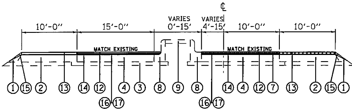
TYPICAL SECTION STA 199+77.66 TO STA. 225+07.50
