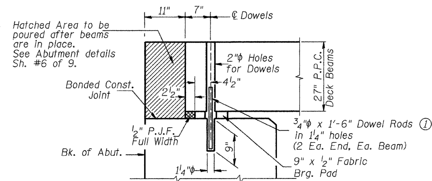
SECTION THRU ABUTMENT (At Right Angles)
