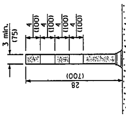
FLEXIBLE DELINEATOR
