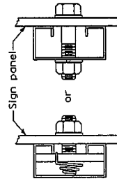
DETAIL C
