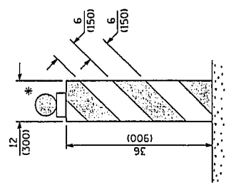
VERTICAL BARRICADE
