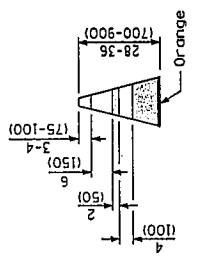
REFLECTORIZED CONE
