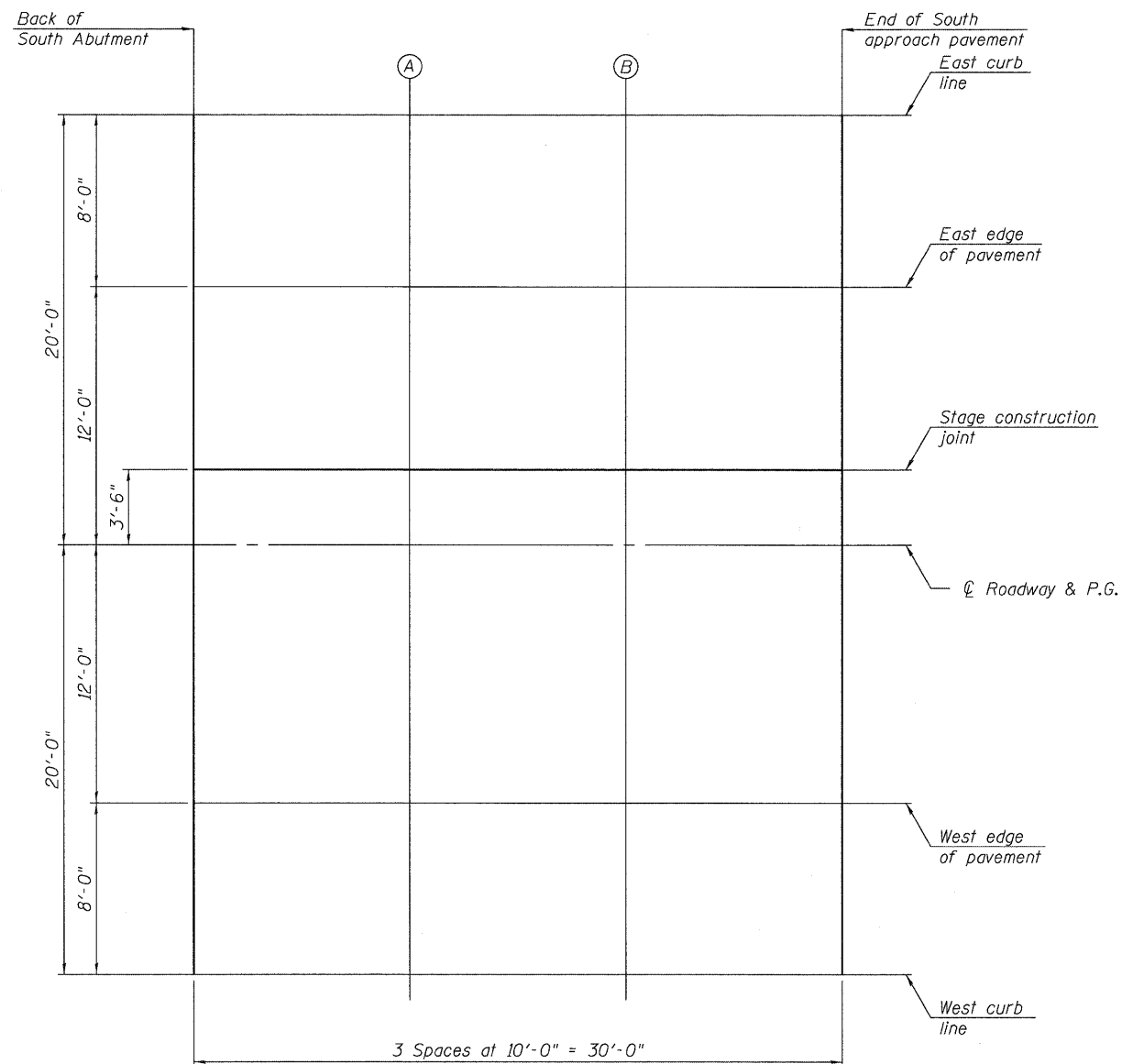
PLAN
