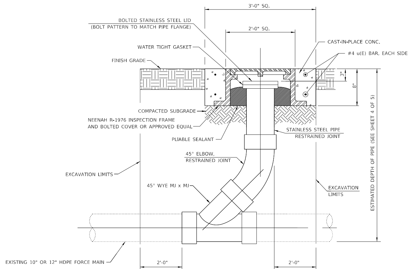
CLEANOUT DETAIL
