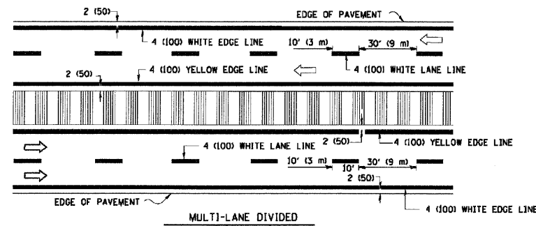
NOTE: MEDIANS WITH BARRIER CURBS DO NOT REQUIRE AN EDGE LINE TYPICAL LANE AND EDGE LINE MARKING
