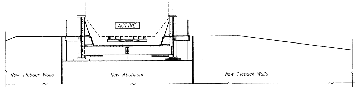
SECTION A-A THRU STAGE 4
