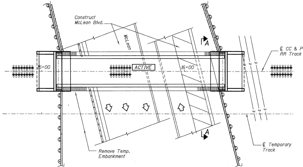
STAGE 4 - RECONSTRUCT McLEAN BLVD.
