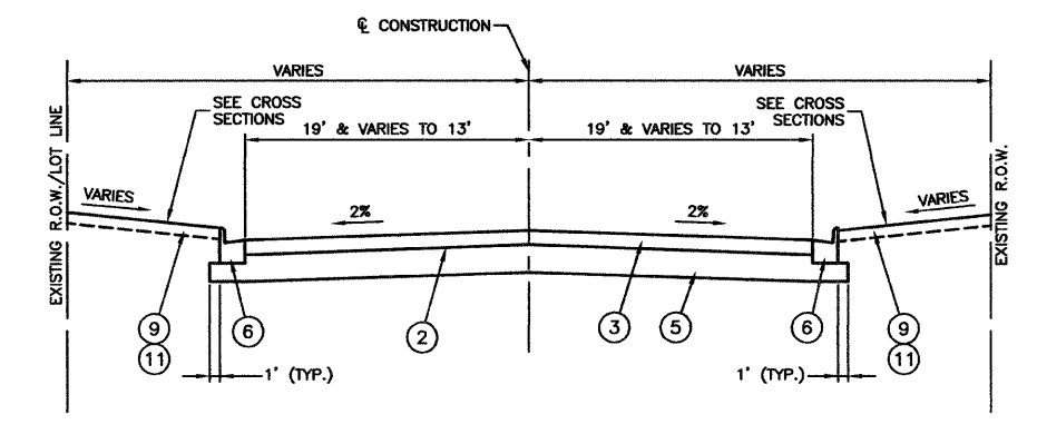
PROPOSED TYPICAL CROSS SECTION
