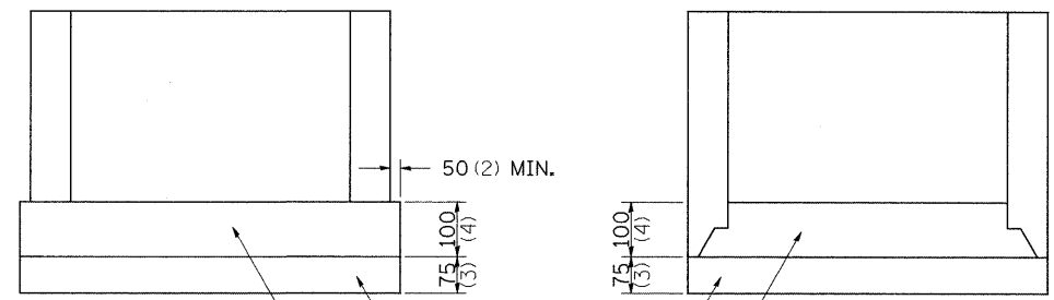
PRECAST REINFORCED CONCRETE SLAB
