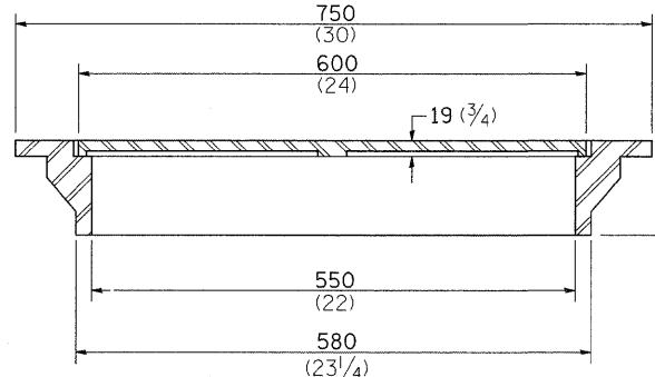
TOTAL WEIGHT: 66 Kg (146 lbs)
