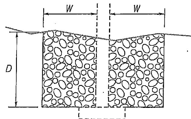
TYPICAL PIER ELEVATION
