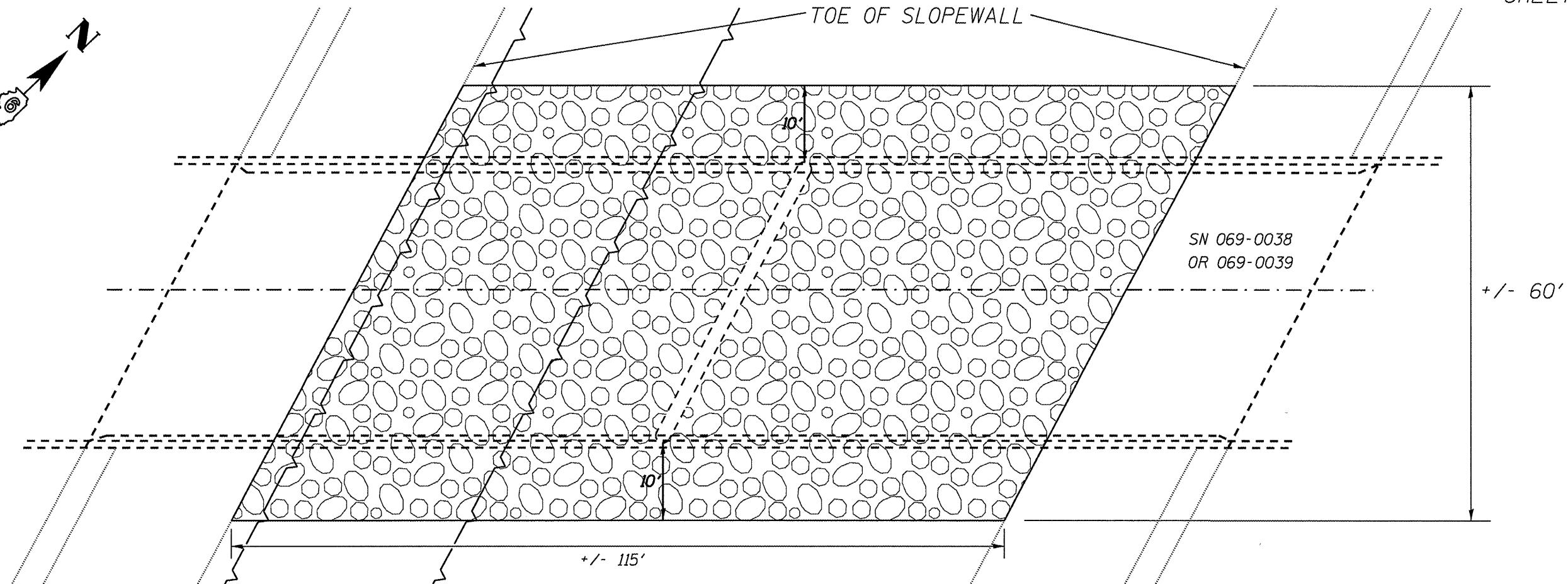
TYPICAL RIPRAP PLAN
