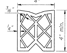
PREFORMED JOINT SEAL
