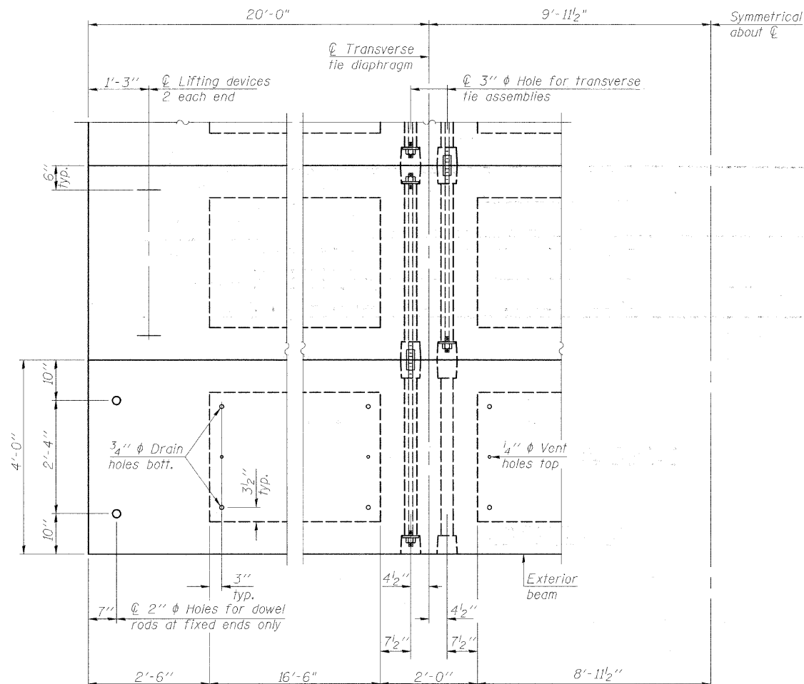
PLAN VIEW
