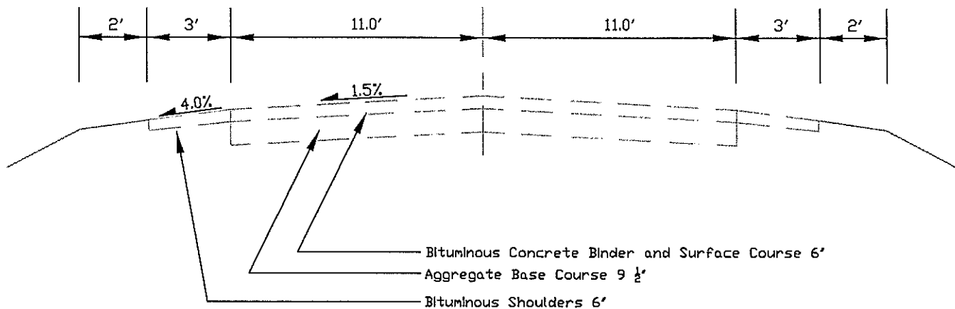
EXISTING TYPICAL SECTION Original Construction Section: 88-00030-04-RS STA. 173+26.00 TO STA. 390+50.00
