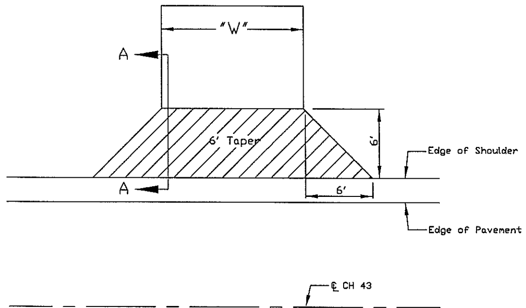
PRIVATE ENTRANCE DETAIL
