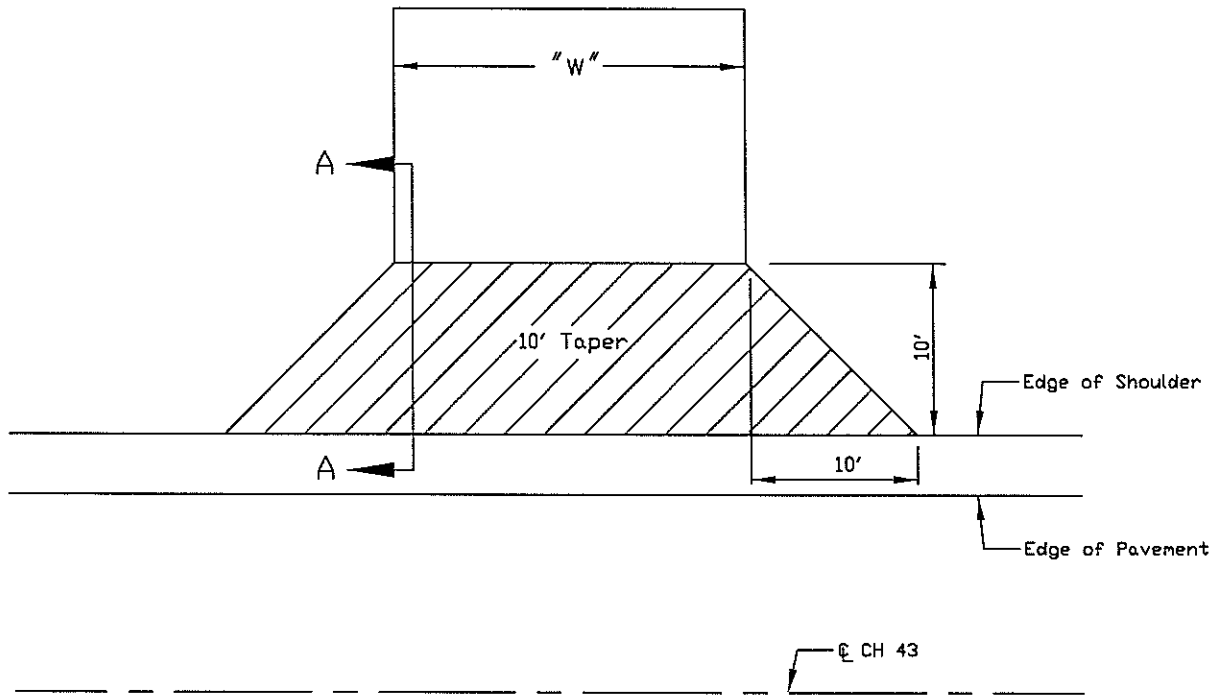
SIDE ROAD INTERSECTION DETAIL
