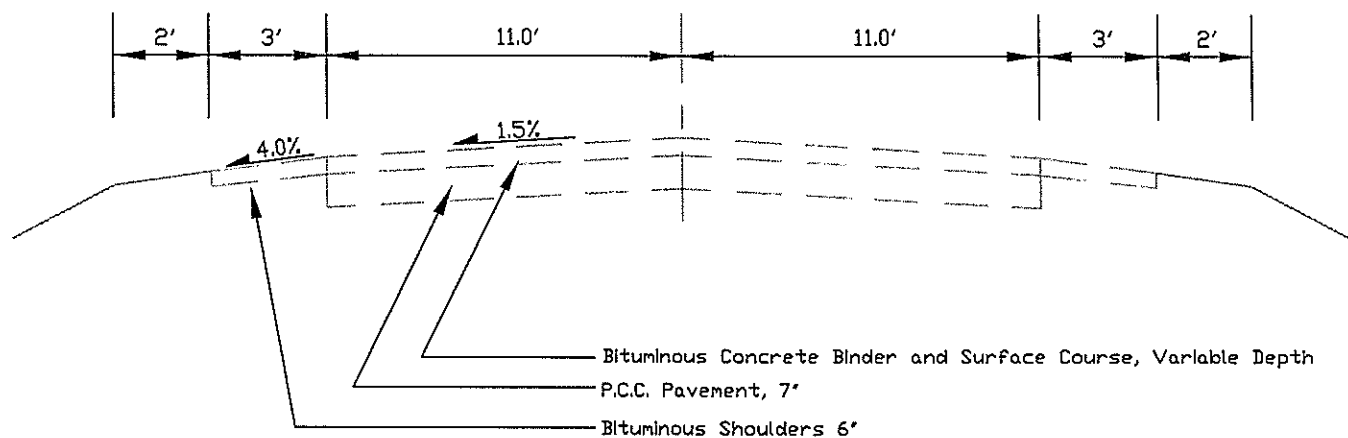
EXISTING TYPICAL SECTION STA. 390+50.00 TO STA. 395+72.50
