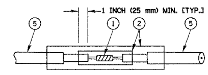
DETAIL "A" LOOP-TO-LOOP SPLICE
