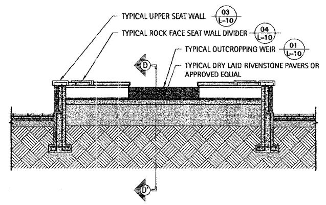
3 Fountain Section B-B' Scale: 1/4" = 1'-0"
