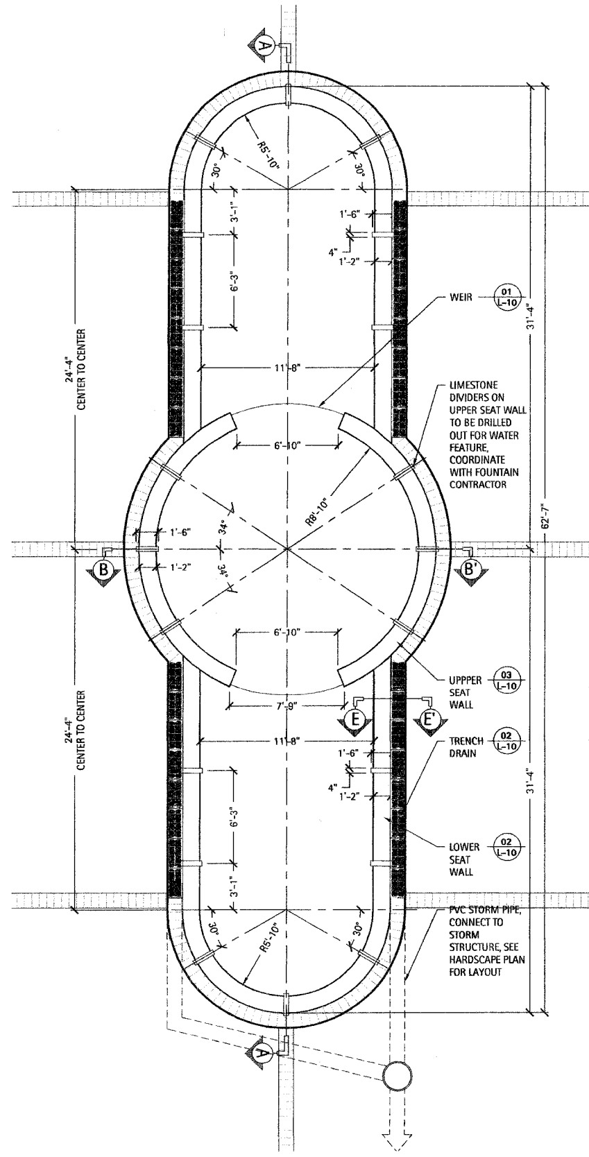
1 Fountain Plan Scale: 1/4" = 1'-0"
