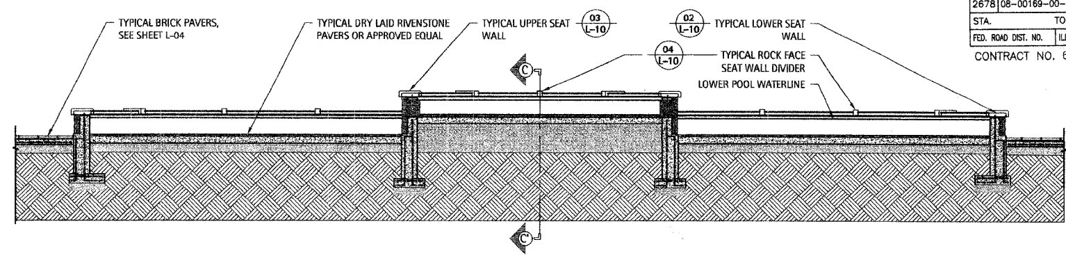
2 Fountain Section A-A' Scale: 1/4" = 1'-0"
