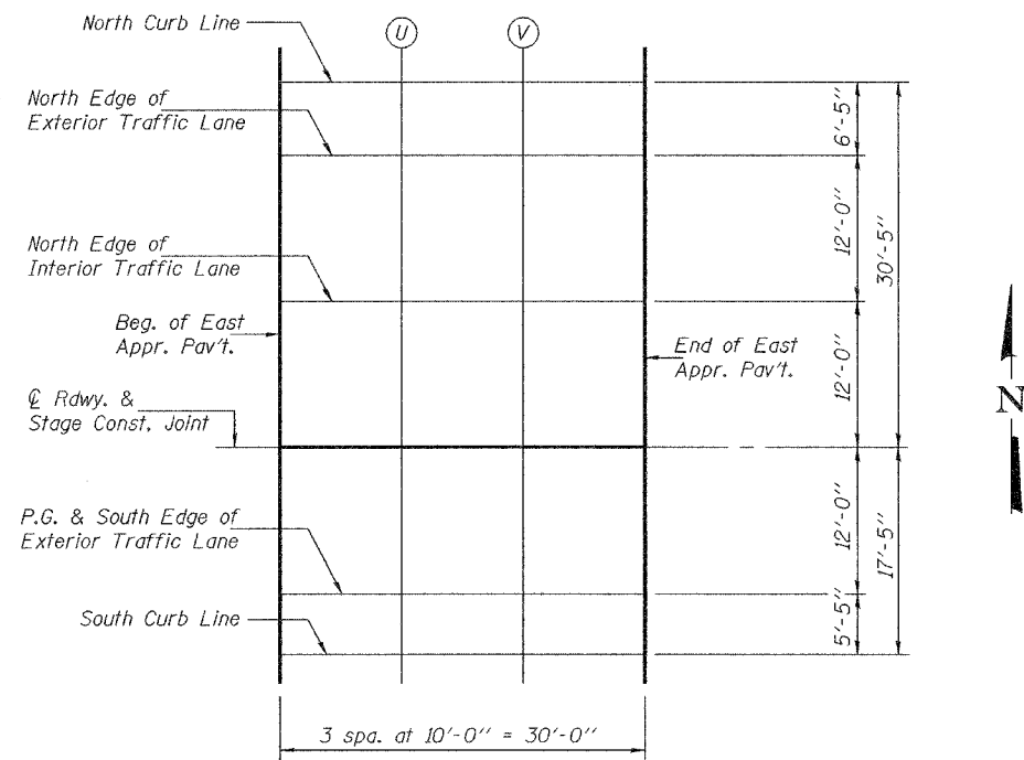
PLAN East Approach (W.B.)
