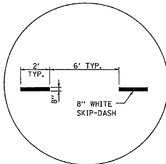
TURN LANE STRIPING
