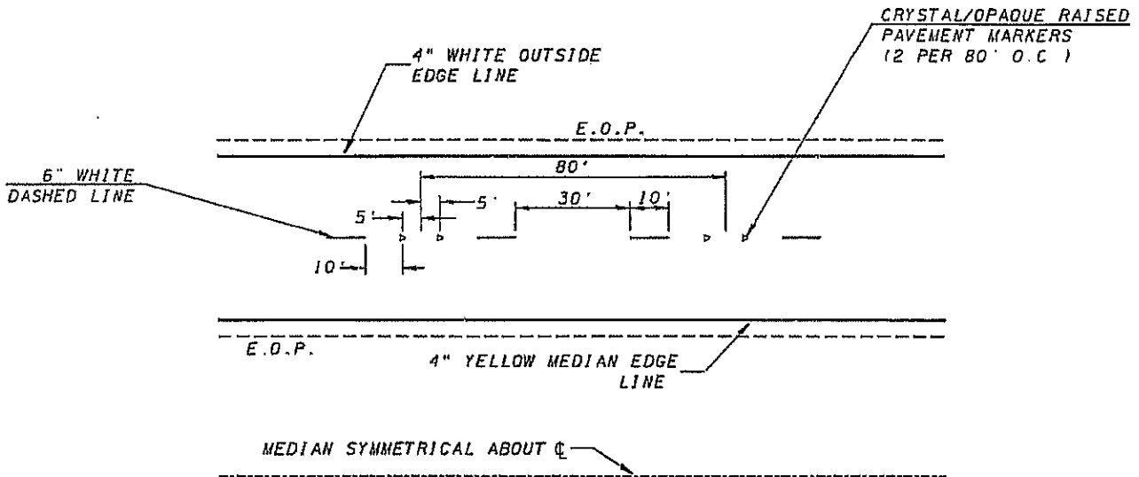
RAISED PAVEMENT MARKER DETAIL
