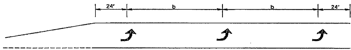
TURN LANE ARROW PLACEMENT 150' AND LONGER
