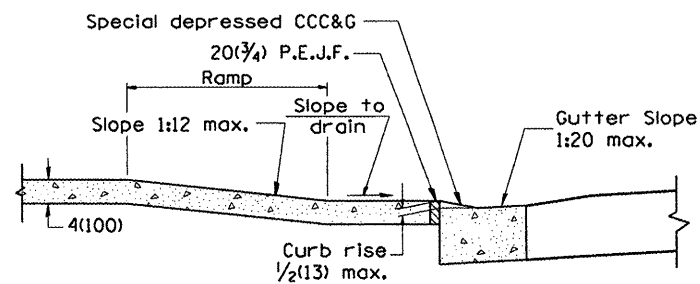
SEC. G-G
