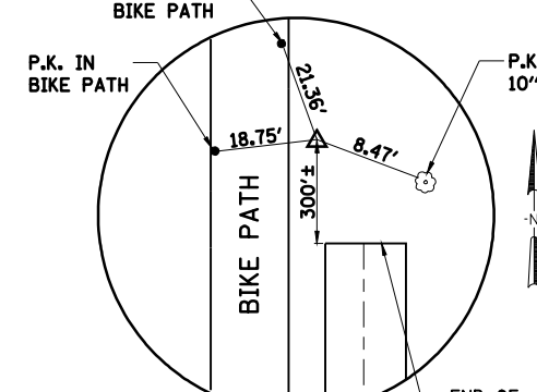
MAC PT8, SET 5/8" IRON PIN STA 841+08.82 @ MACARTHUR BLVD.
