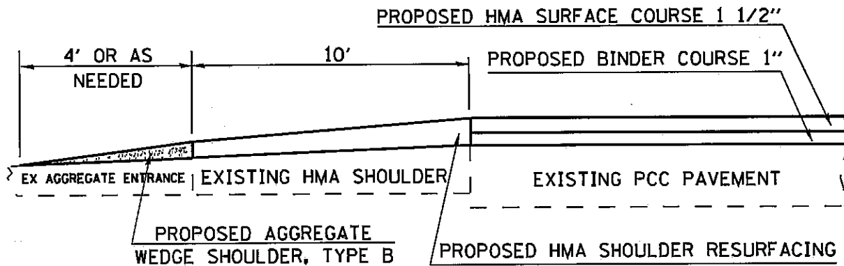
AGGREGATE WEDGE DETAIL FOR AGGREGATE ENTRANCES
