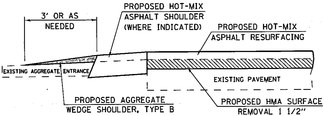
AGGREGATE WEDGE DETAIL FOR AGGREGATE ENTRANCES
