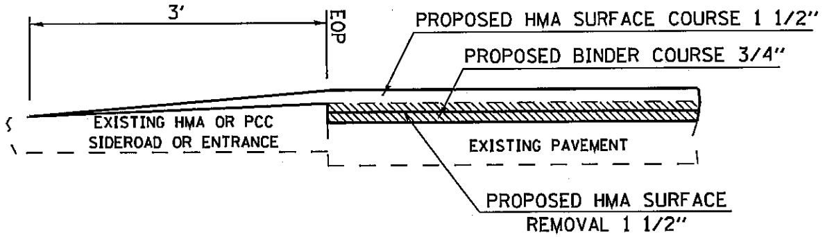
FEATHEREDGE DETAIL FOR OIL AND CHIP, HOT-MIX ASPHALT, AND CONCRETE SIDEROADS AND ENTRANCES
