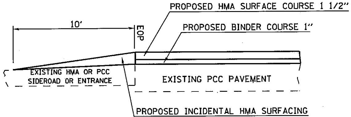
FEATHEREDGE DETAIL FOR OIL AND CHIP, HOT-MIX ASPHALT, AND CONCRETE SIDEROADS AND ENTRANCES
