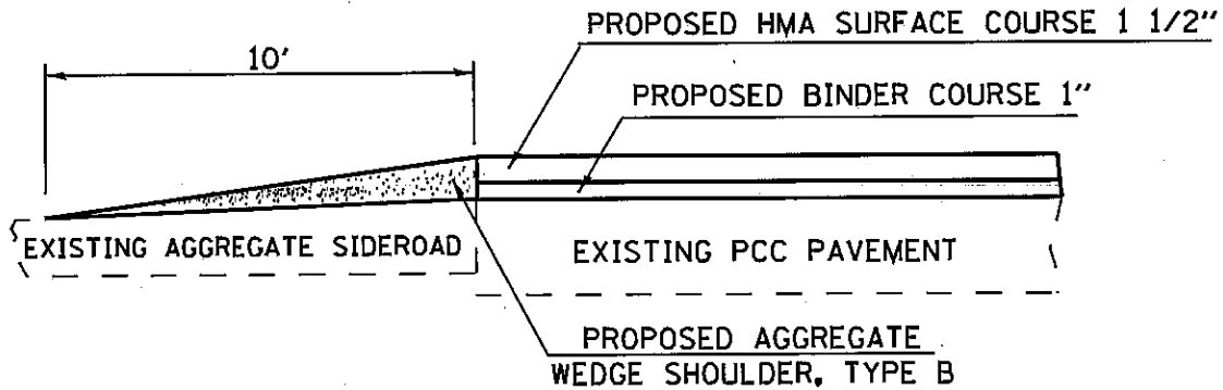
AGGREGATE WEDGE DETAIL FOR AGGREGATE SIDEROADS
