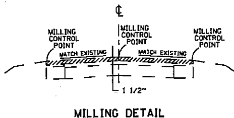
MILLING DETAIL
