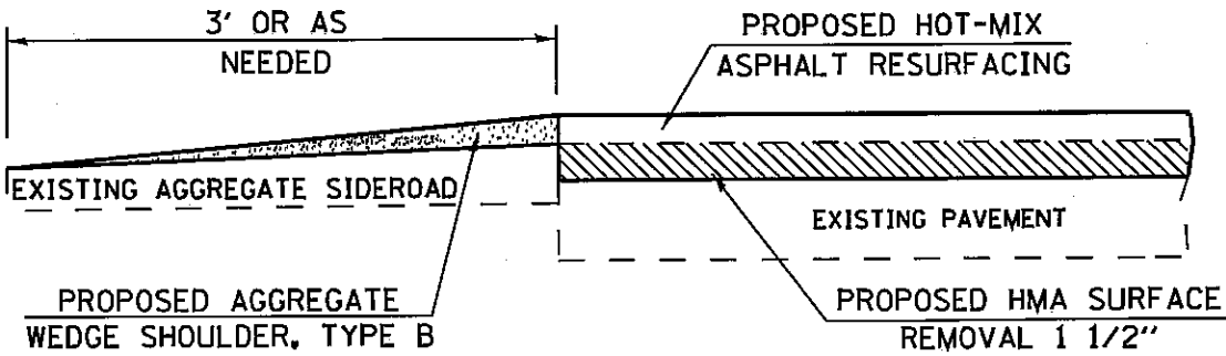
AGGREGATE WEDGE DETAIL FOR AGGREGATE SIDEROADS
