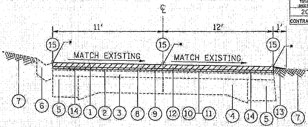
EXISTING TYPICAL SECTION MILE 0.467 TO MILE 0.540
