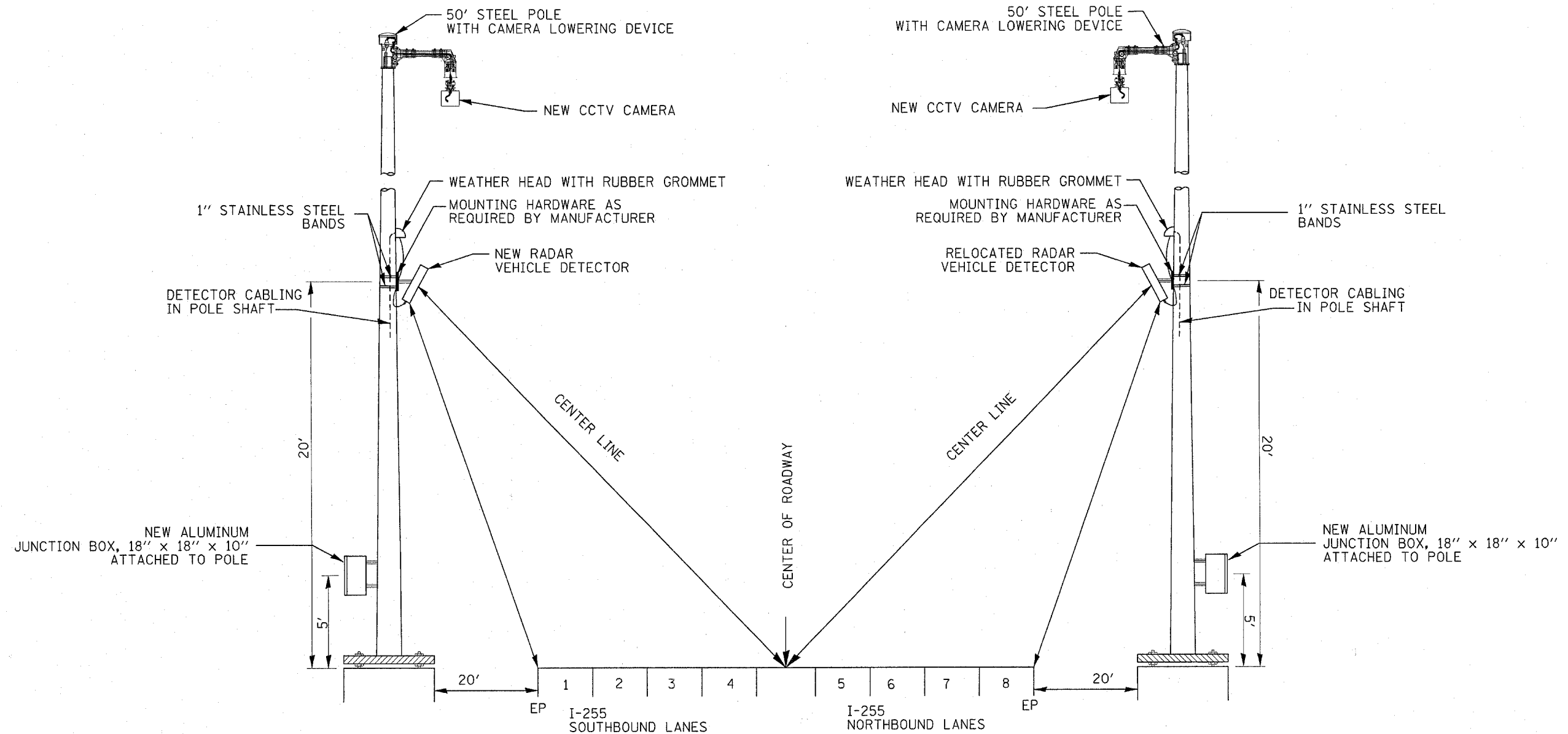
DETAIL RADAR VEHICLE DETECTOR NOT TO SCALE
