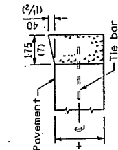
DEPRESSED CURB
