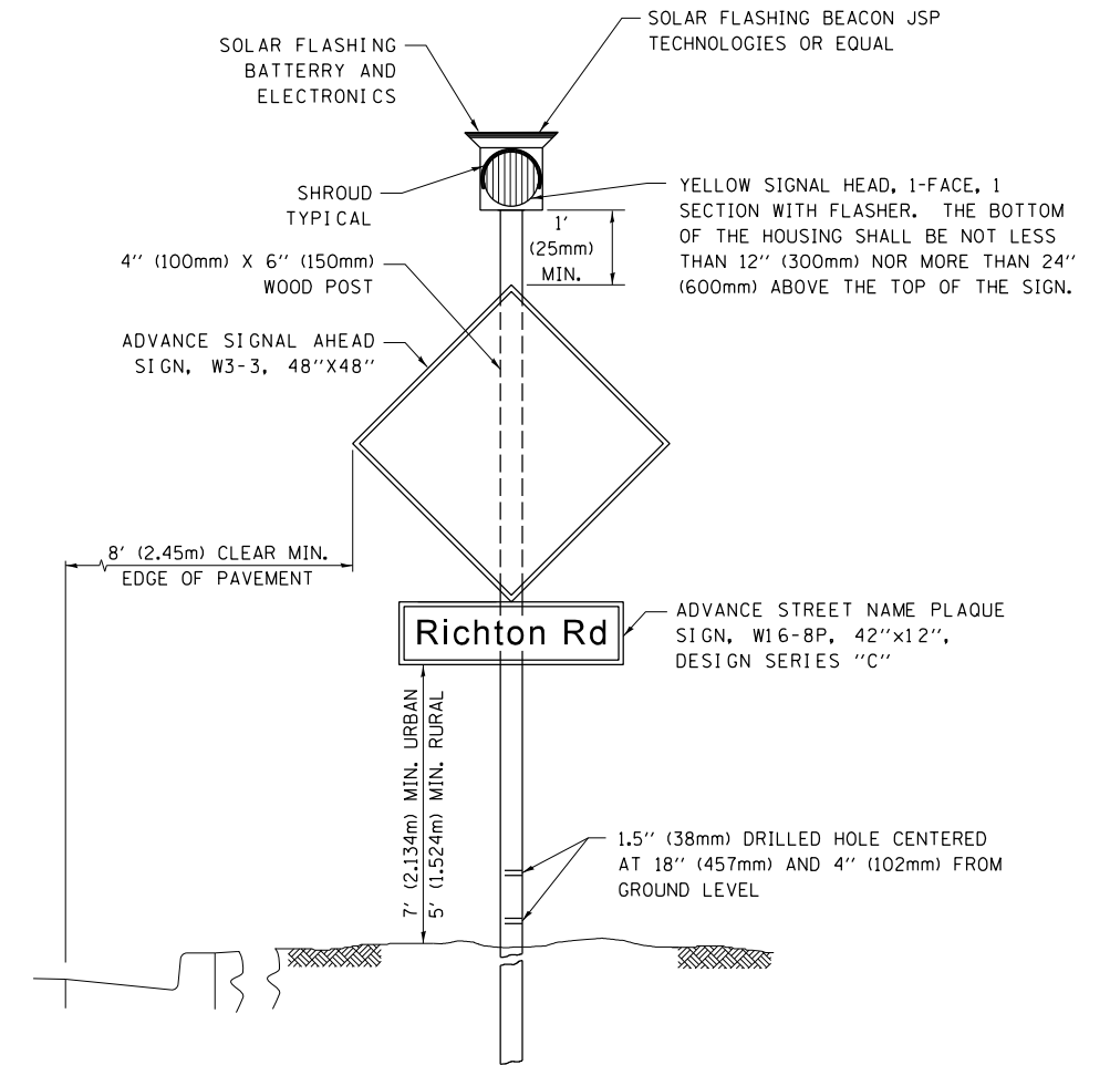
PROPOSED SOLAR FLASHER (24-HR) DETAIL (NOT TO SCALE)
