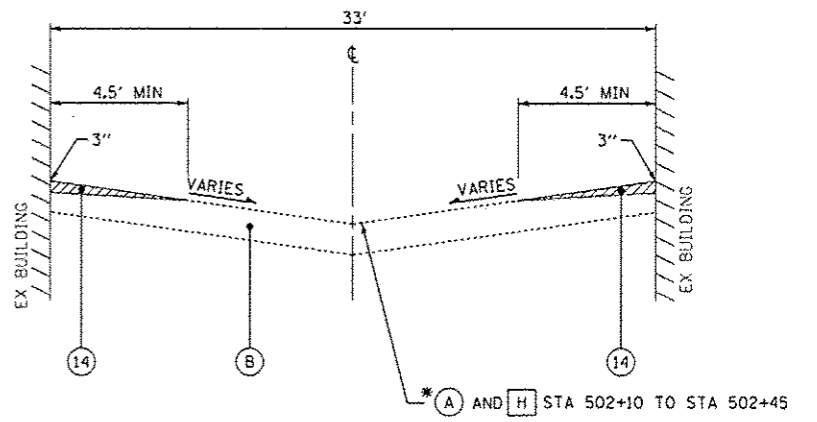
EXISTING TYPICAL SECTION ROAD 5 STA 500+19 TO STA 502+45
