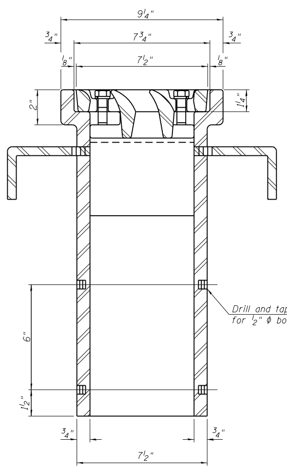
SECTION B-B
