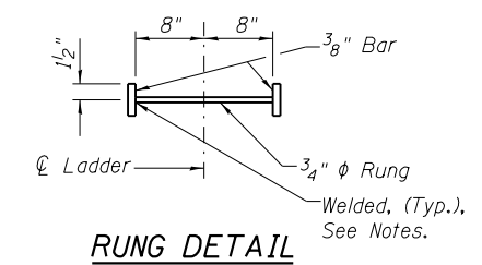
DETAIL I
