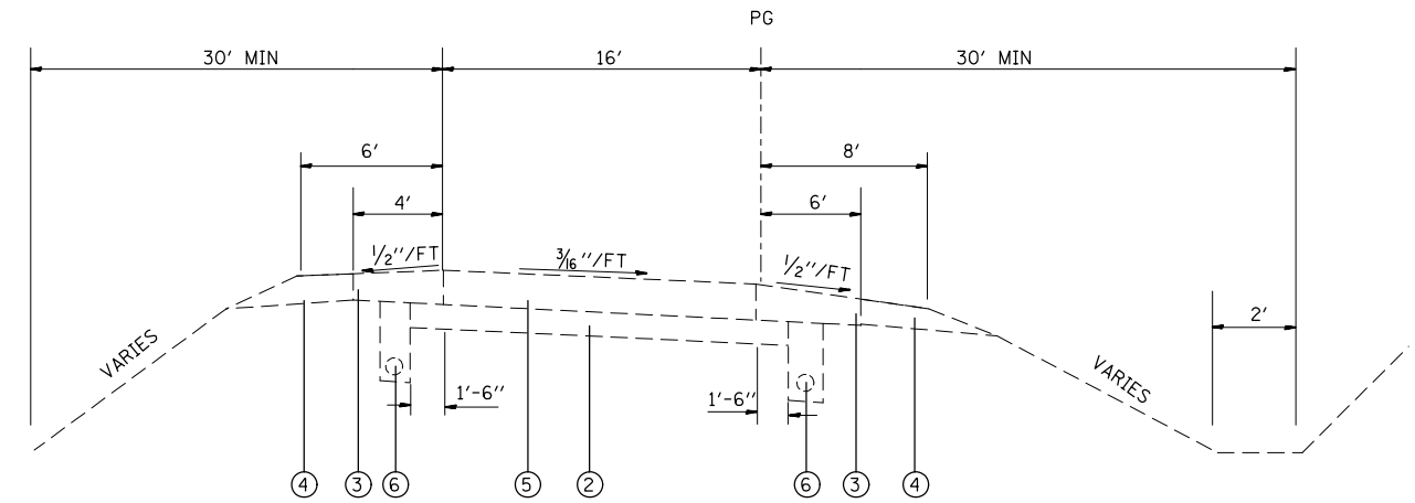
TYPICAL SECTION RAMP TANGENT
