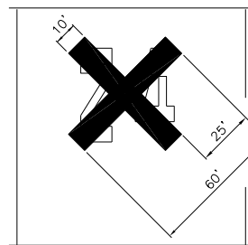
ON PAVEMENT CLOSED RUNWAY MARKER DETAIL N.T.S.
