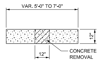
PROFILE VIEW
