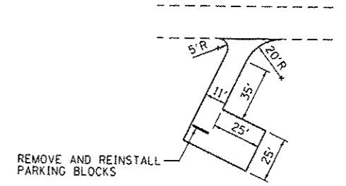
PLAN - TYPICAL CAMPSITE N.T.S.
