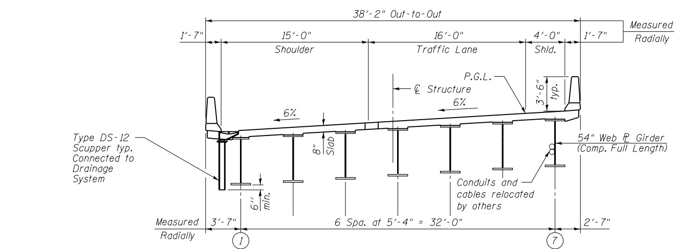
TYPICAL CROSS SECTION - FINAL (Looking West)
