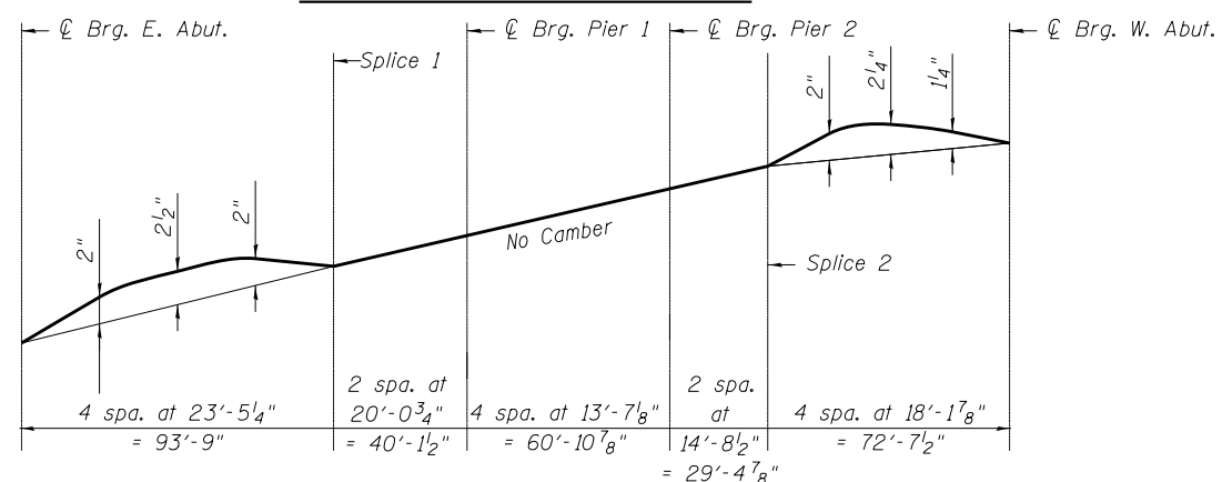
GIRDER 3 CAMBER DIAGRAM
