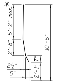
BARS v 310 (E) * Cut in Field to Fit
