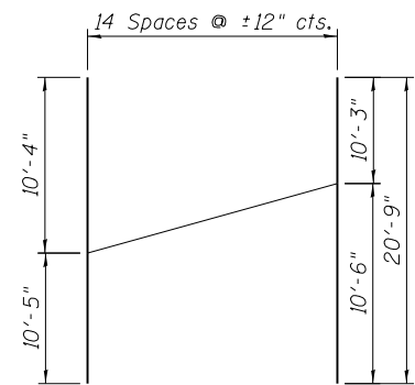
BAR v 324 (E) BAR CUTTING DIAGRAM * Order Bars Full Length, Cut to Fit
