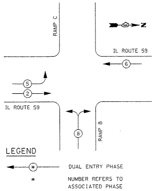
TEMPORARY PHASE DESIGNATION DIAGRAM PRESTAGE, STAGE 1, STAGE 1A, STAGE 1B
